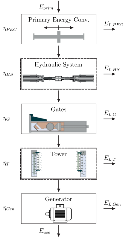
Fig. 2: Illustration of the energy conversions in the plant
