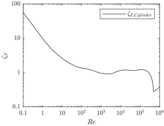
Fig. 6: \zeta_F of cylindrical body as a function of Re (see Figure 4-119 in [3])
