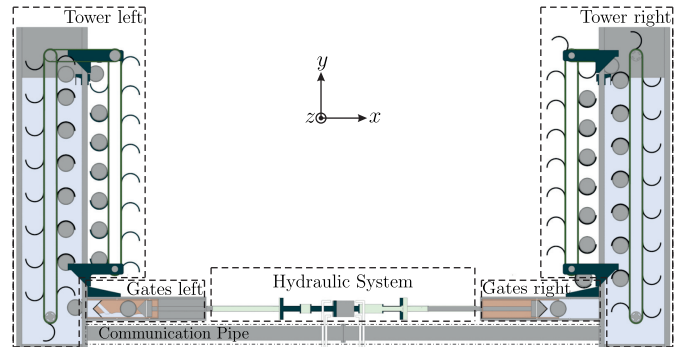
Fig. 1: Schematic illustration of the plant
