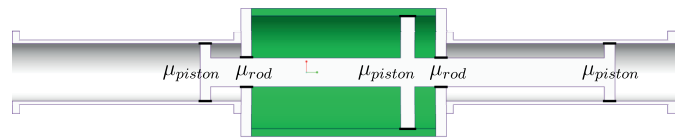
Fig. 4: Friction contacts working cylinder
