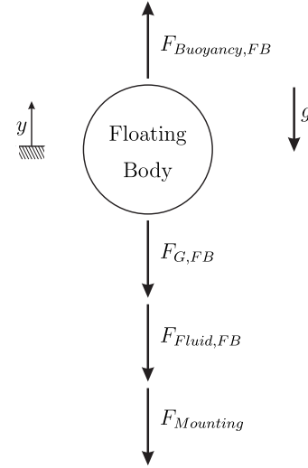
Fig. 5: Free punch floating body
