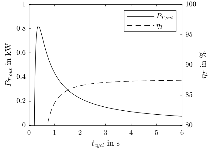
Fig. 7: Tower power and efficiency as a function of cycle time
